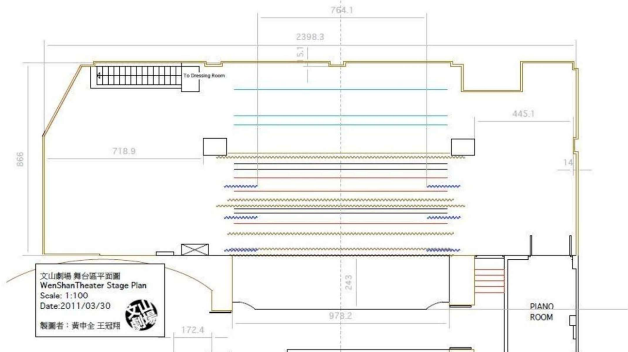
舞台區基本空間示意圖 Diagram and Dimensions of Acting Area
